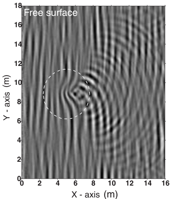
Fig. 3 Numerical simulation of the free surface elevation for Case 3 (narrow-directional spread)
