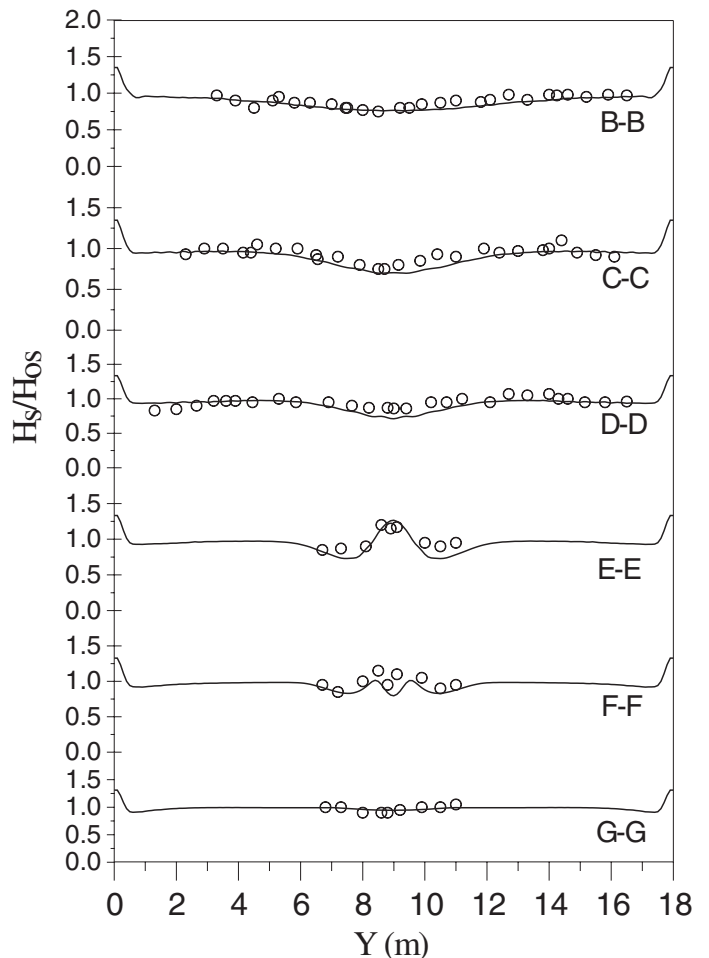
Fig. 5 Normalized significant wave heights along the transects shown in Figure 2 for Case 6 (Broad directional spread). Experimental data: o o o; numerical data (OLUCA-SP): —. Dissipation model: Thornton and Guza (1983) ( B = 1.0 and \gamma = 0.6 ).
