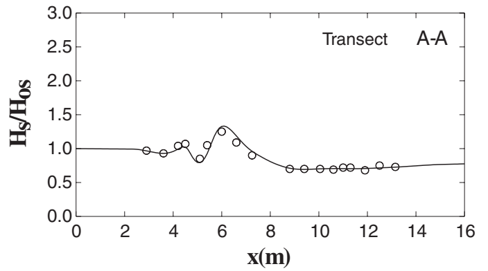
Fig. 4 Normalized significant wave heights along transect A-A for Case 6. Experimental data: o o o; numerical results (OLUCA-SP): —. Dissipation model: Thornton and Guza (1983) ( B=1.0 and \gamma=0.6 ).
