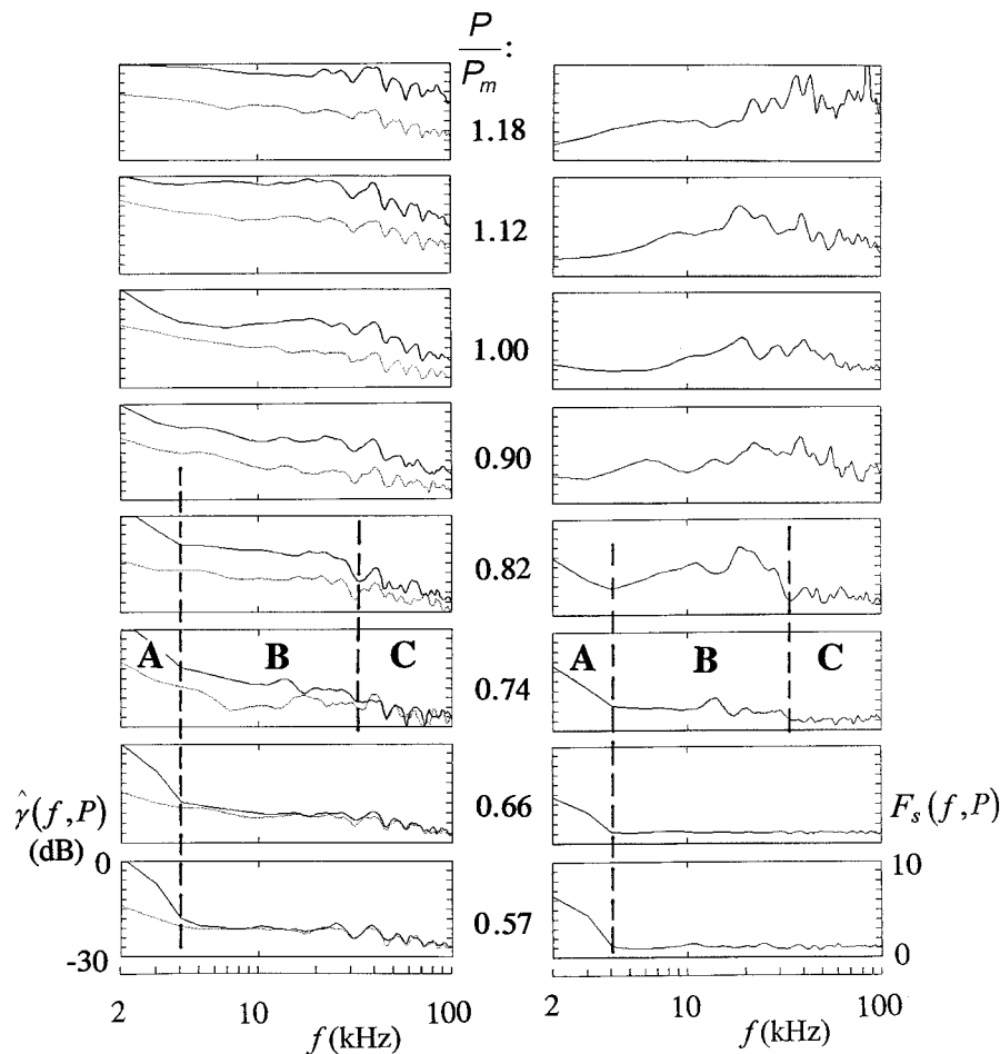
Fig. 10 Peak-selective spectra (left) and spectral crest-factor (right) derived from the same signals, sensed at the power P . B and C are identified as the mechanisms 1 and 2 described in Fig. 1, 6, and 9.
