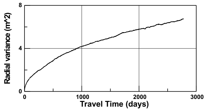
Fig. 5 Radial variance of the particle displacements around their mean in case of homogenized aquifer under advection and dispersion processes.
